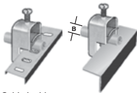
Cable Ladder Cross Rung
