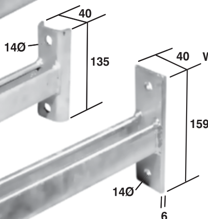
3 FLAT PLATE ARM (254 SERIES)
