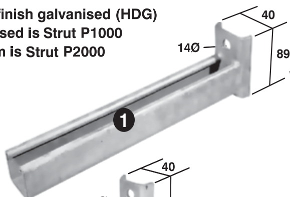
1 89mm WRAP AROUND (223 SERIES)
