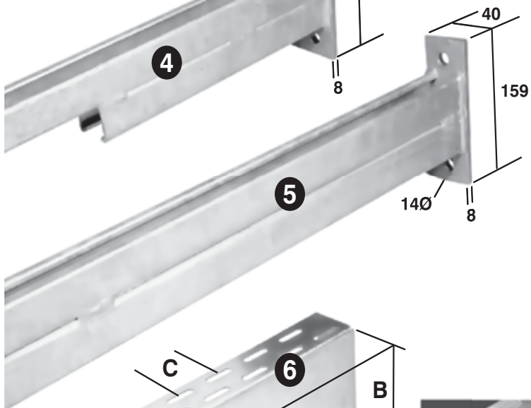
5 FULL DOUBLE (254 SERIES)
