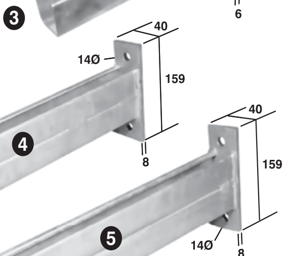
4 HALF DOUBLE (254 SERIES)
